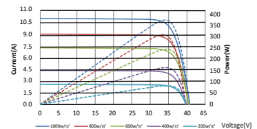
Current-Voltage Curve (BSM375M-60HPH)
